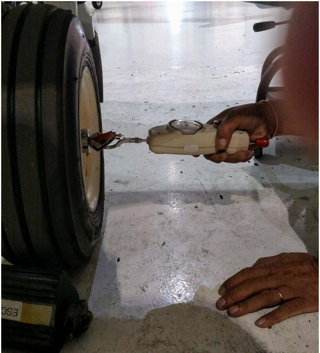
Figure 3. WST Pull Test
